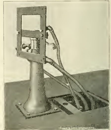
FIG. 2. AIR PUMP TESTING RACK IN VERTICAL POSITION, SHOWING PIPE CONNECTIONS.
